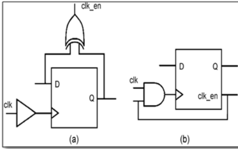
Fig. 7. Enabling of the Clock Signal.
