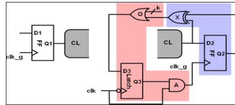
Fig. 9. Application of Clock Gating With Feedback Enabling Signals. The Components Highlighted In Red Centered Shaded Area Comprise The Clock Gater, While Those In Blue Reside In FF.
