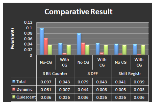
Fig. 11 Comparative results of power reduction With clock gating and without clock gating
