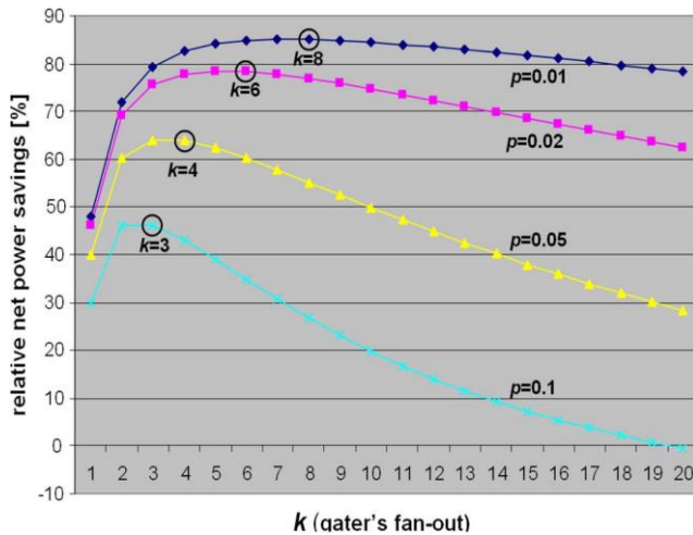
Fig. 9. Normalized power net savings per FF obtained by adaptive gating at 1st level of clock tree in (6). The savings is compared to the non gated situation. The optimal fan-out is marked for each toggling probability.
