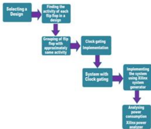
Fig. 10 Design flow of Proposed technique
