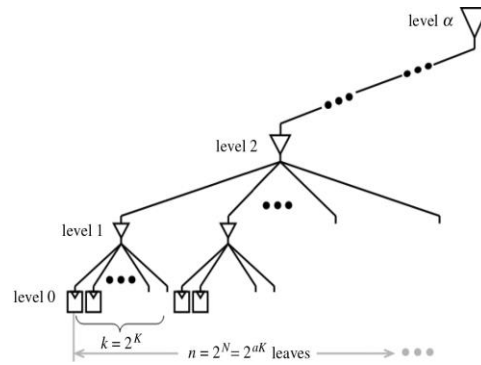
Fig. 6. Sized clock tree distribution network.
