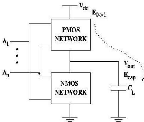
Fig. 5 General CMOS transistor circuit
