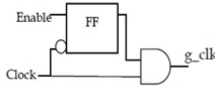
Fig. 2 Flip flop based clock gating Cell
