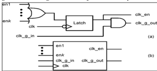
Fig. 8. Joining K Enabling Signals Generated By Distinct Flip-Flops Into One Gating Signal.
