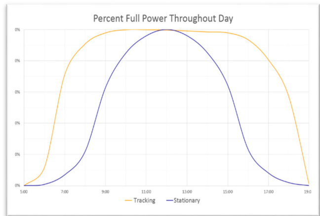
Fig.4. Typical Power curve of Stationary Vs Tracking system
